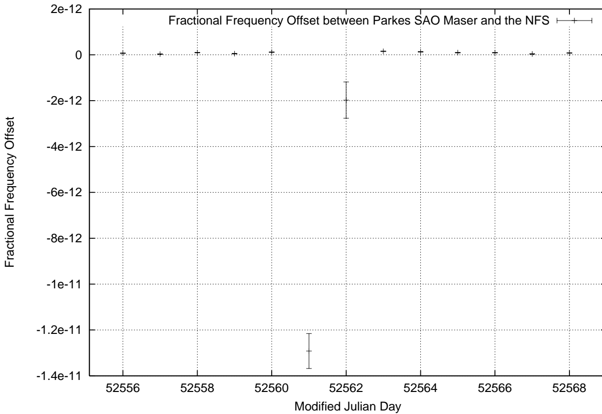
GPS Common-View Frequency Transfer between ATNF Parkes and NML Sydney
