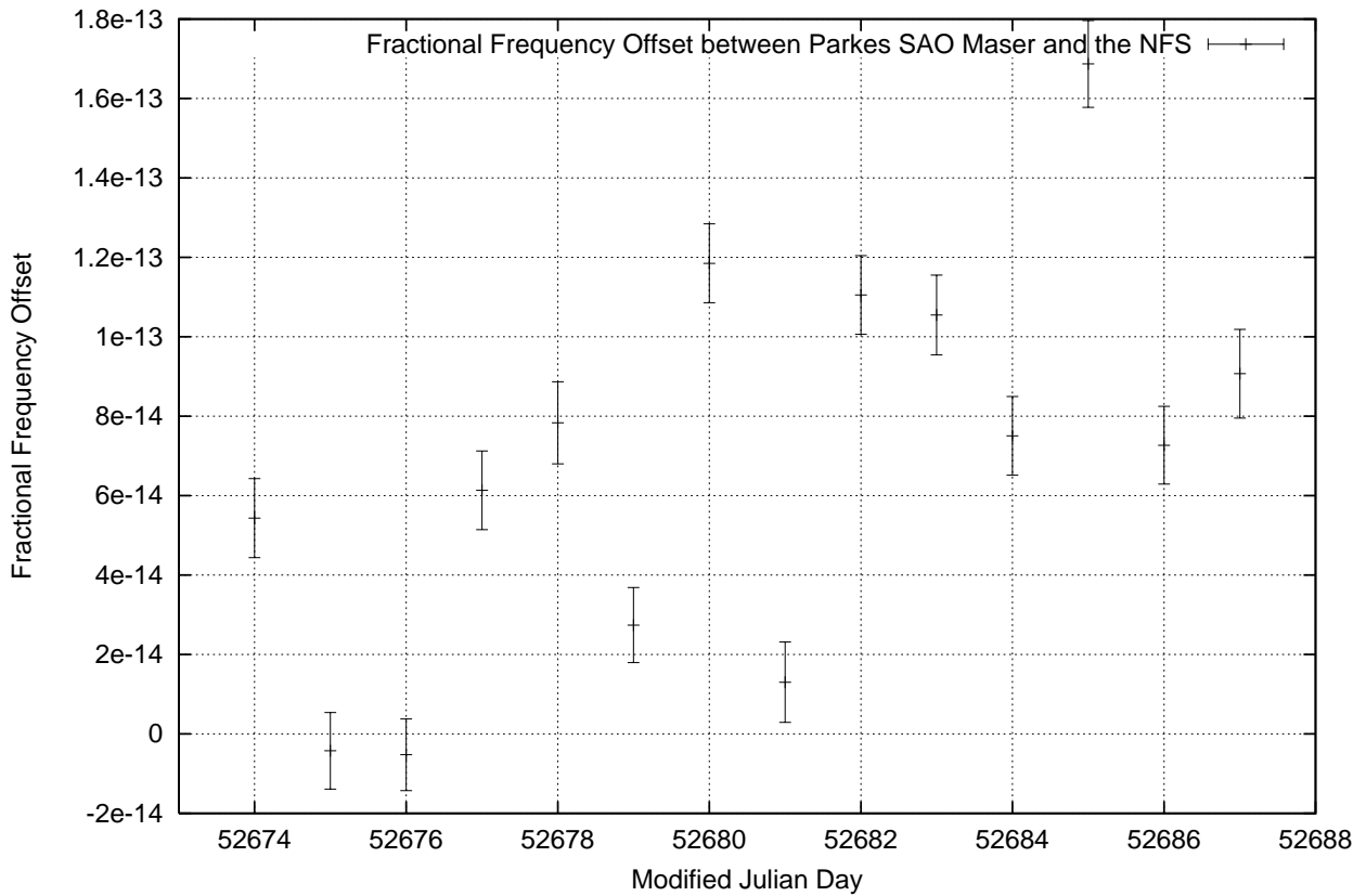
GPS Common-View Frequency Transfer between ATNF Parkes and NML Sydney
