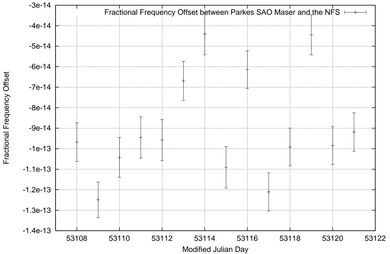
GPS Common-View Frequency Transfer between ATNF Parkes and NML Sydney
